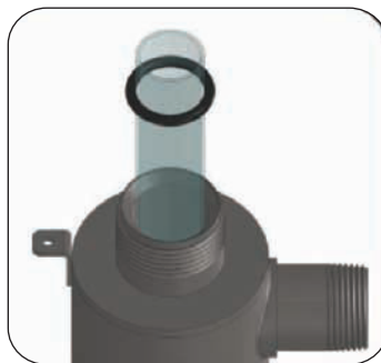
Figure 4. Quartz Sleeve installation
